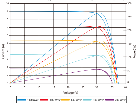
Current-Voltage & Power-Voltage Curve (265)
